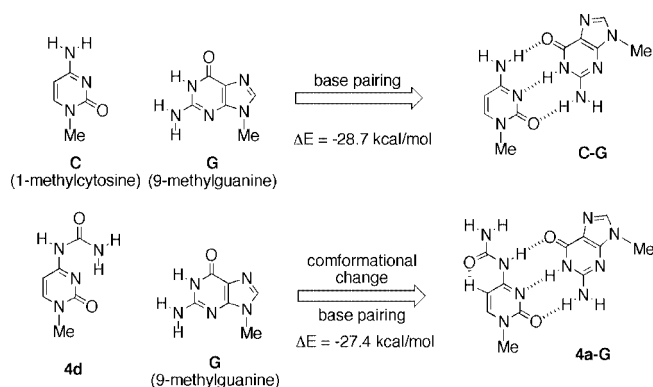
Figure 8. Predicted Watson–Crick base pair between 4- N -carbamoyl-dC and dG. The hydrogen-bonding energy ( \Delta E ) including the energy loss of conformational change is also indicated.
